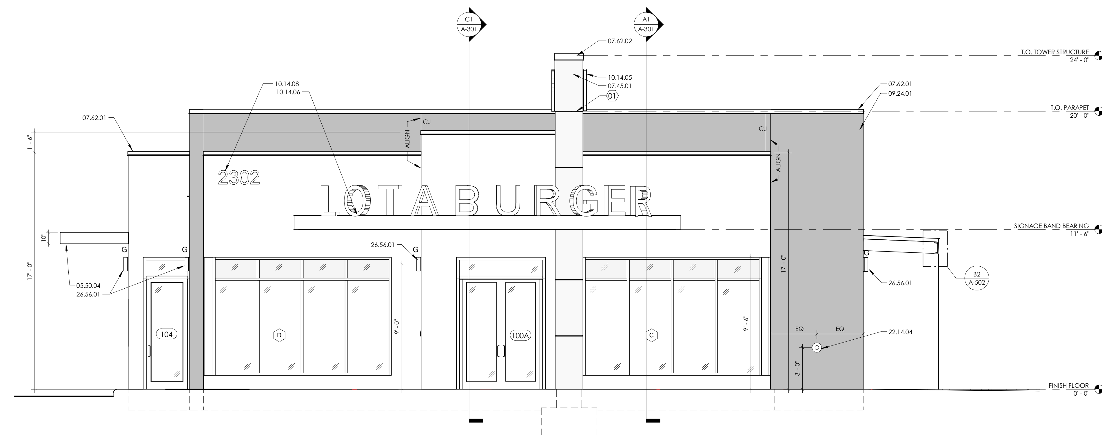
(C1) WEST ELEVATION 1/4" = 1'-0"
