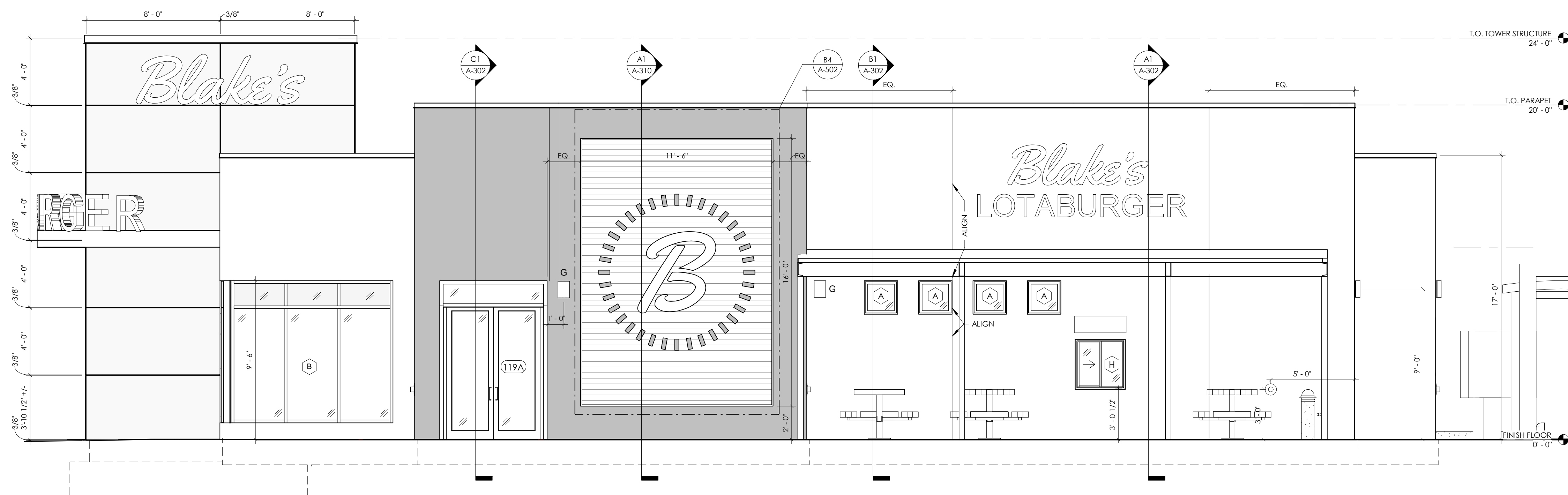
(A1) SOUTH ELEVATION 1/4" = 1'-0"
